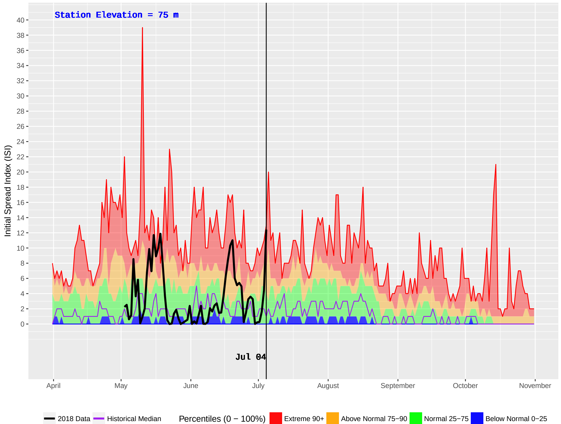
KITPARK (106) : Historical (1995–2016) and Current (2018) Noon Initial Spread Index (ISI)
