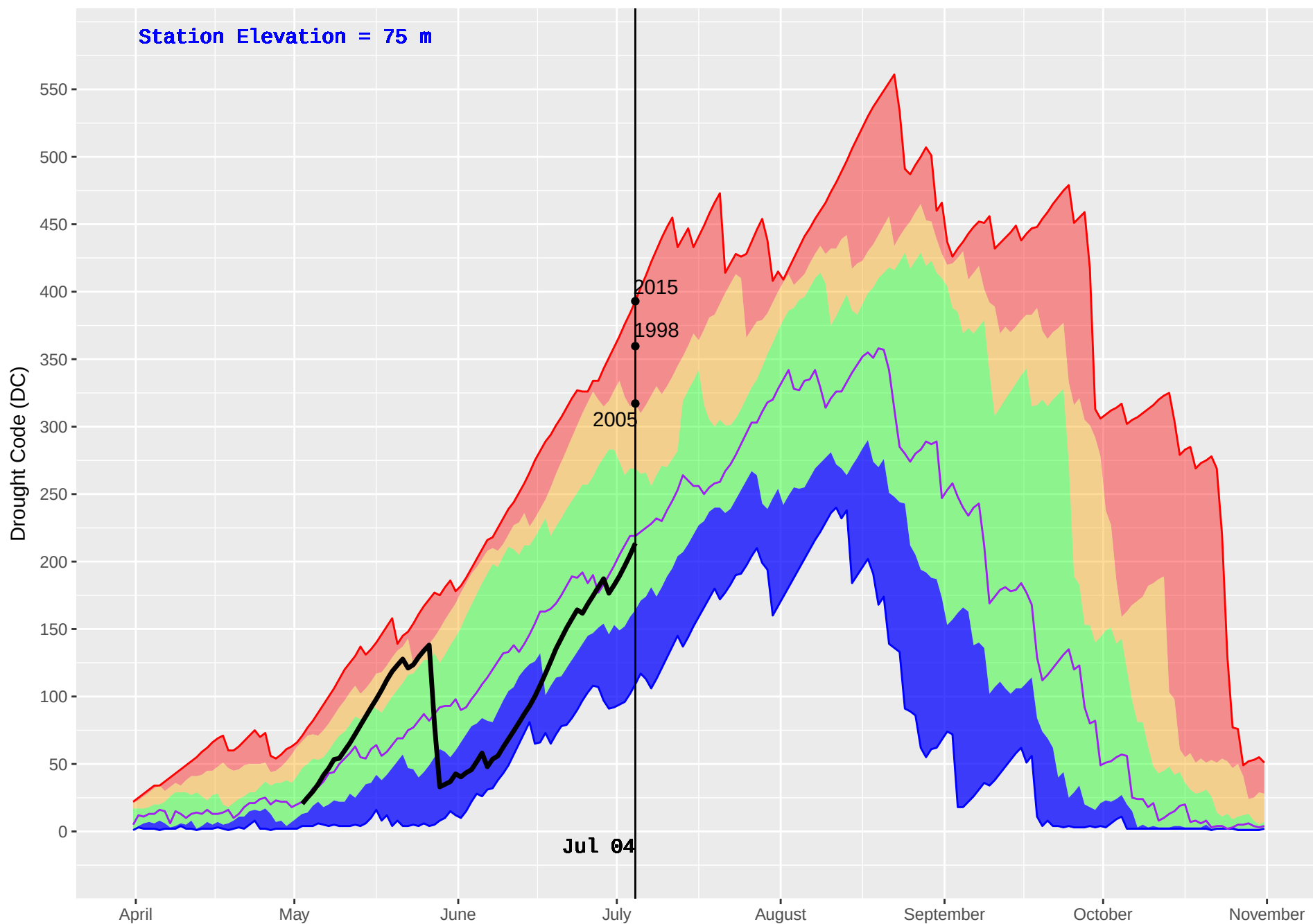
KITPARK (106) : Historical (1995–2016) and Current (2018) Noon Drought Code (DC)
